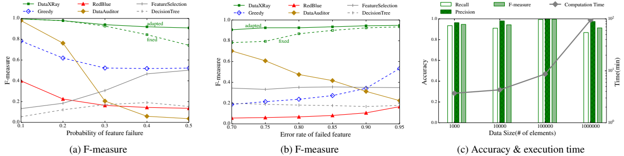
Figure 7: Performance of different methods when we vary the parameters of our synthetic data generator. (a) and (b) show the robustness of DATAXRAY whereas (c) shows the scalability of our parallel implementation of DATAXRAY.
