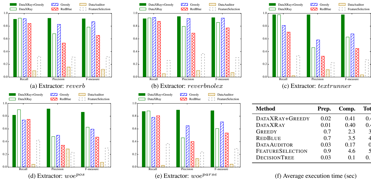
Figure 5: The quality of the derived diagnoses for all of the methods, across five knowledge extraction systems; the maximum F-measure value achieved by DECISIONTREE was 0.0148, which was too low to display in the graphs. Our approach that combines DATA XRAY with a greedy set-cover step outperforms all other approaches, in some cases significantly. It is also faster than other methods except DATA AUDITOR and DECISIONTREE, but the latter two produce results of very low quality for our problem.
